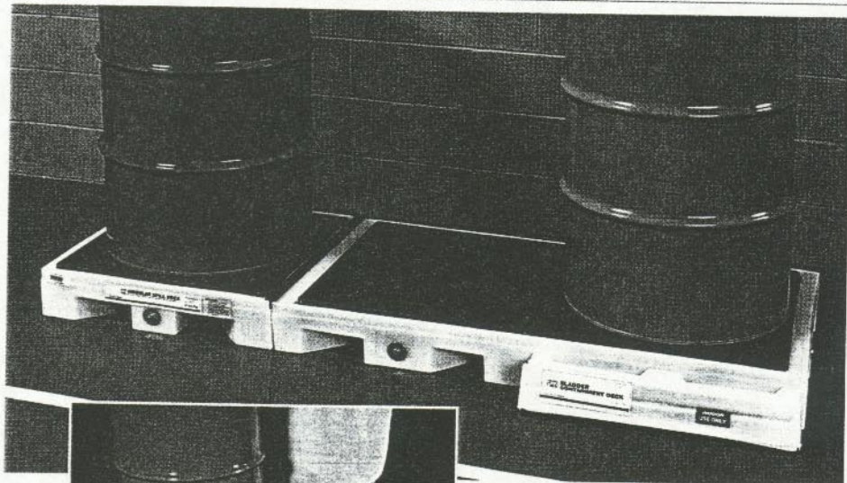
Attached Bladder Box provides 66 gallons of containment—keeps the deck height a low 5 3/4".
